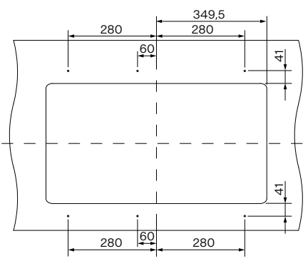
KBK 110-70
