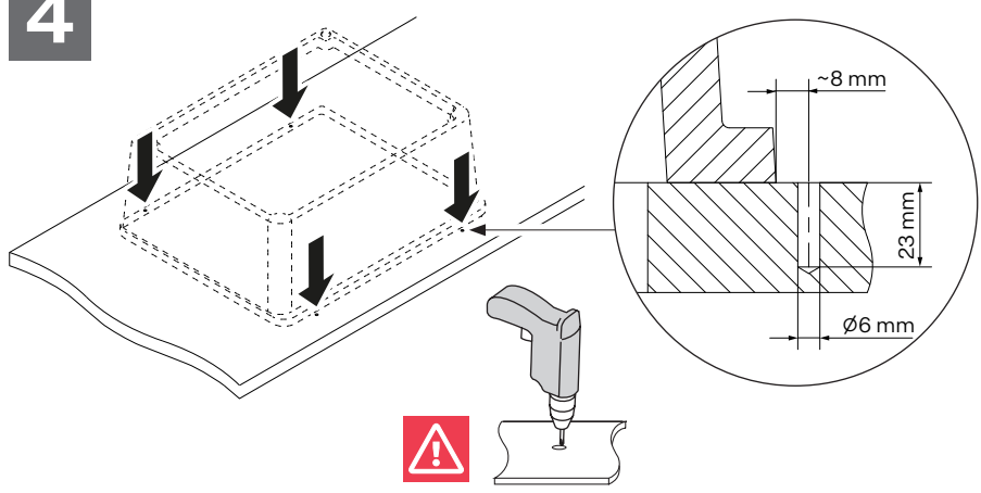
KBK 110-40
